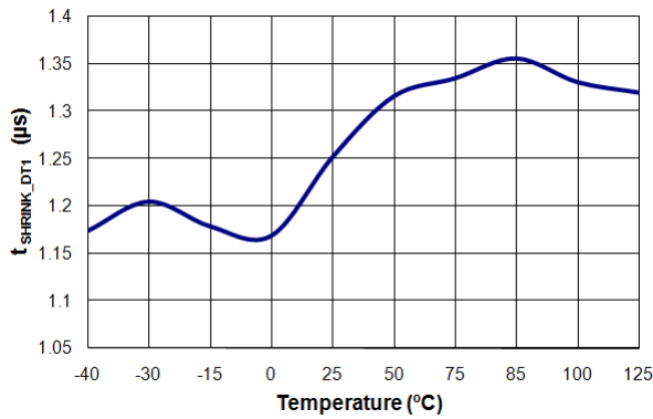
Figure 34. t_{SHRINK\_DT1} vs. T_A
