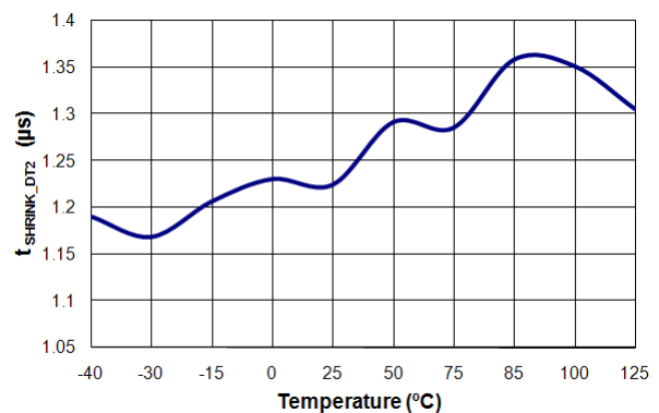
Figure 35. t_{SHRINK\_DT2} vs. T_A
